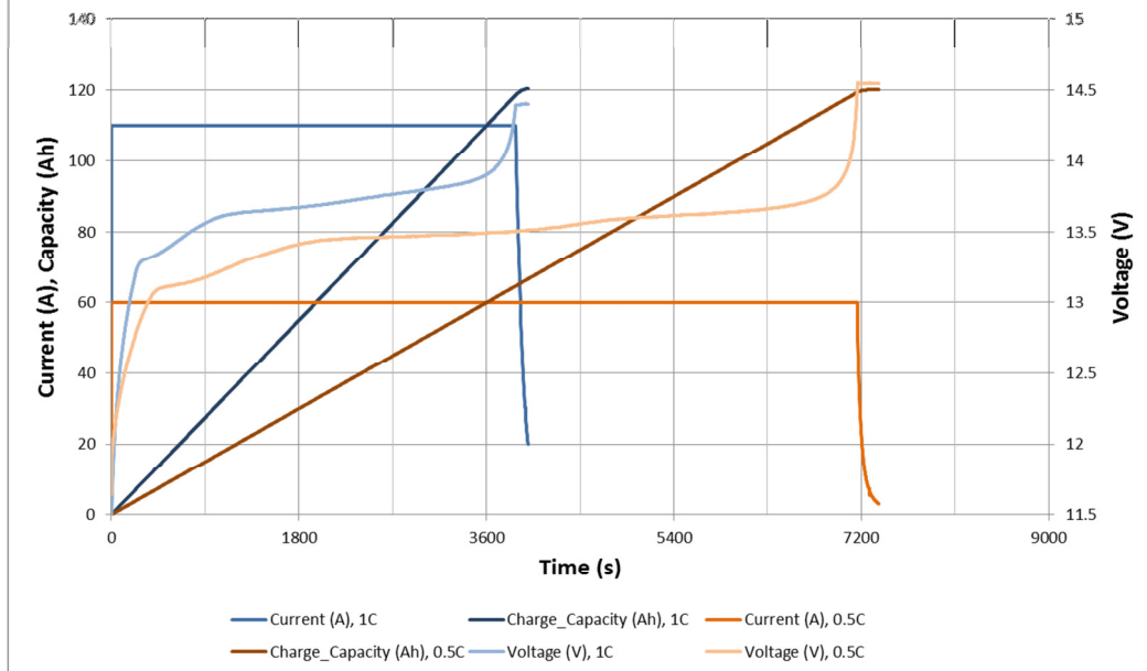
ELP-12V1450Wh Charging Curves, 23°C
