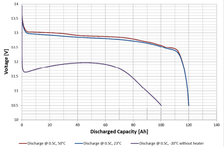
ELP-12V1450Wh Discharge Curves, 0.5C
