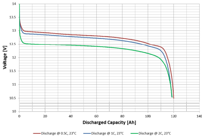
ELP-12V1450Wh Discharge Curves, 23°C
